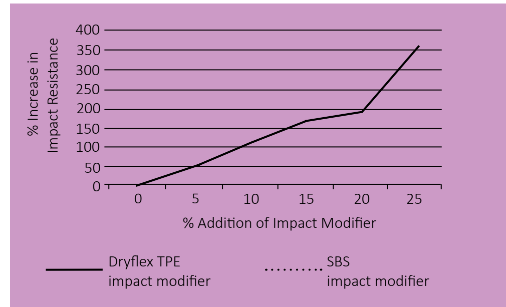
FIGURE 2. INCREASE IN IMPACT RESISTANCE OF POLYSTYRENE REGRIND
